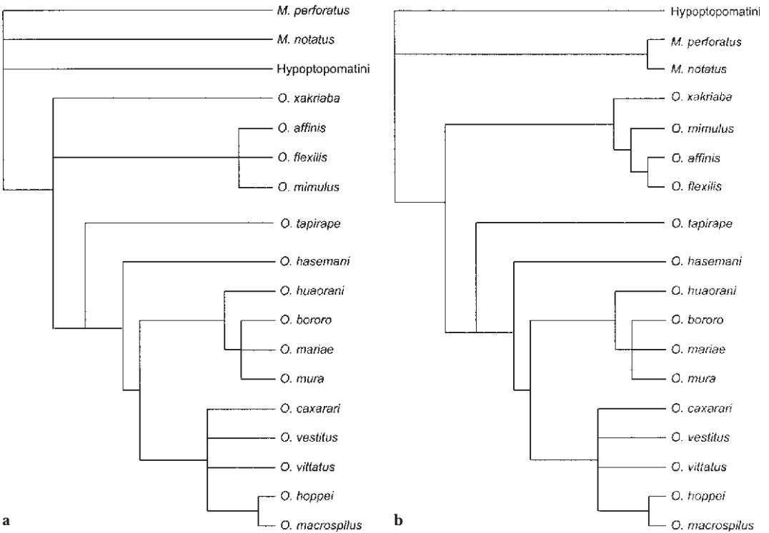
Fig. 4. a , Strict consensus tree of relationships among Otocinclus species, based on Schaefer (1997) and Britto & Moreira (2002), with addition of O. mimulus . Tree length 48 steps, CI=0.6250, RI=0.7907, RC=0.4942. b , Single most parsimonious tree of relationships among Otocinclus species, as (a), but with mimetic relationship with Corydoras species added as character. Tree length 50 steps, CI=0.6200, RI=0.7889, RC=0.4891.
