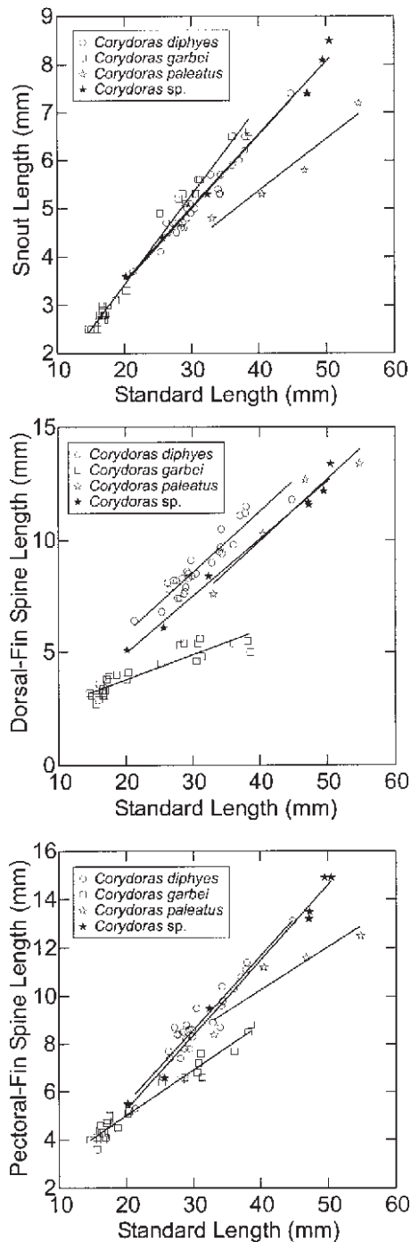
Fig. 7. Snout length, dorsal spine length and pectoral spine length plotted against standard length, showing major morphometric differences between Corydoras diphyes , C. garbei (Tables 8-9), C. sp. aff. ehrhardti . (Table 10), and C. paleatus (Table 11).
